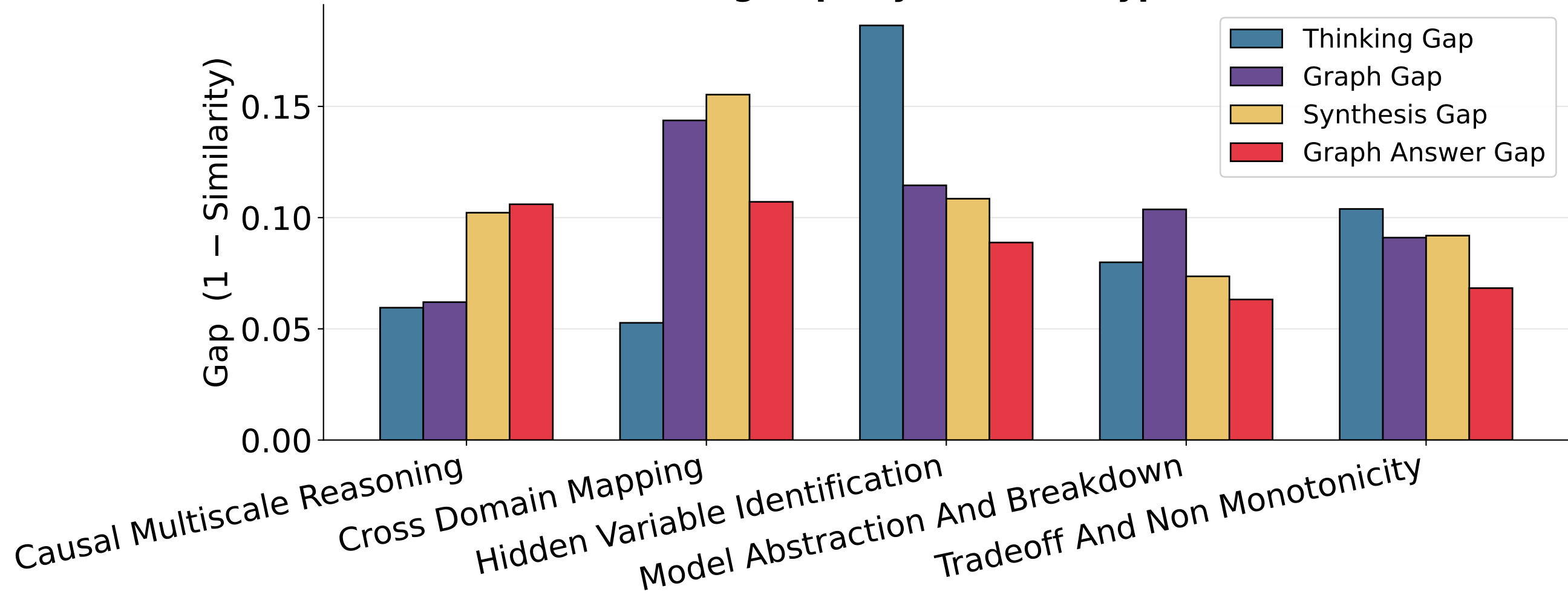
Backtracking Gaps by Question Type (n = 100)
