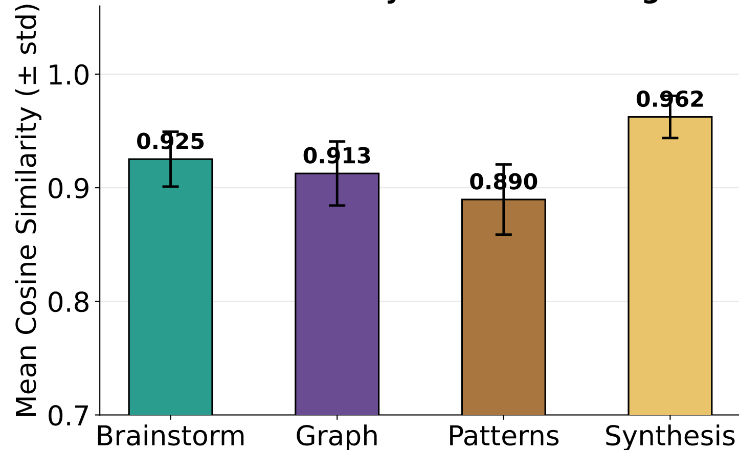
Mean Similarity: Answer vs Stage
