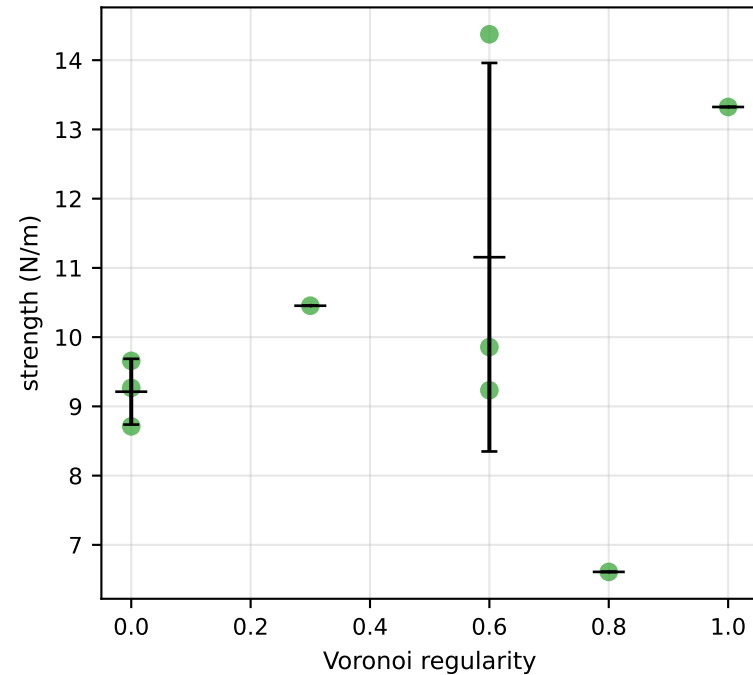
polygonal networks (25 cells): seeds and mean \pm sd
