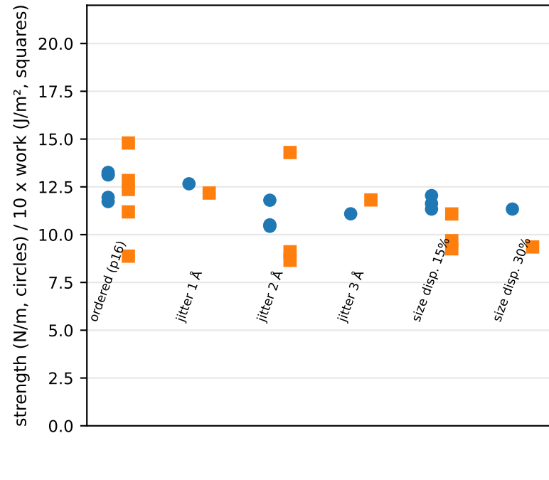
ordered vs disordered pore lattices (individual runs)
