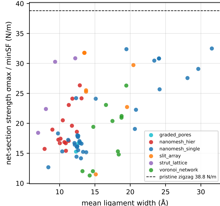
net-section master plot (porous designs)
