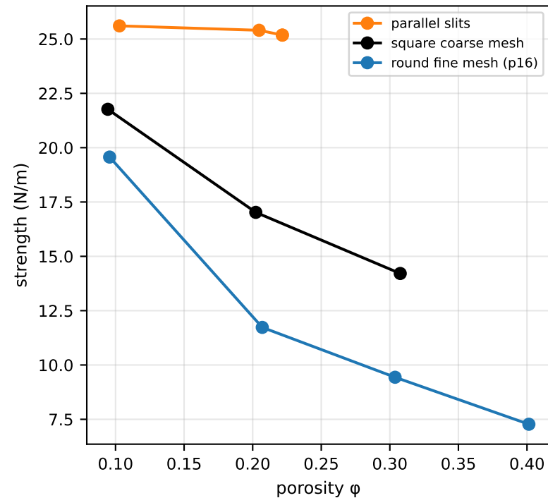
porosity scaling of three architectures
