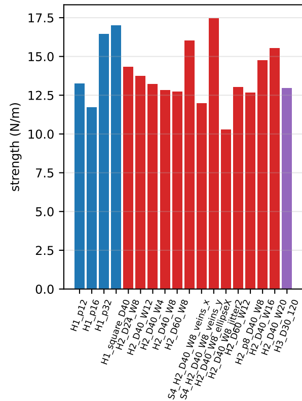
hierarchy ladder at matched porosity \phi \approx 0.20 (blue: 1 level, red: 2 levels, purple: 3 levels)
