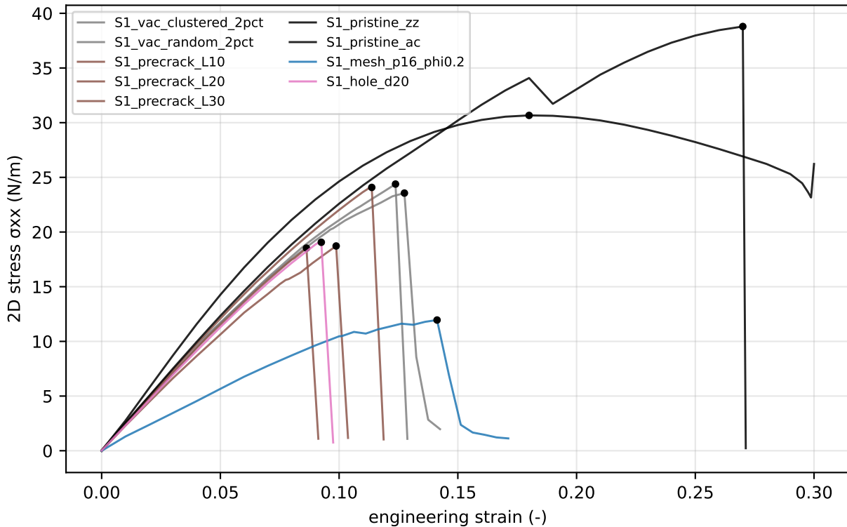
stress-strain curves, stage1_baselines (9 simulations)
