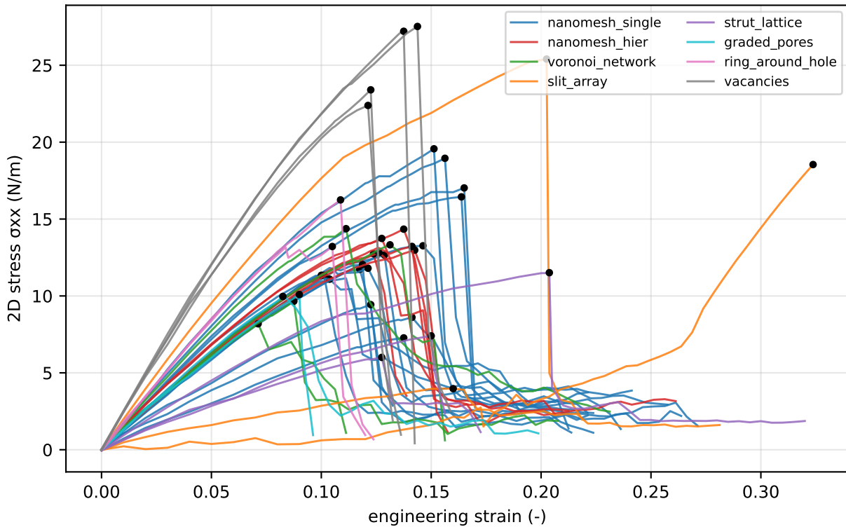
stress-strain curves, stage2_reconnaissance (39 simulations)
