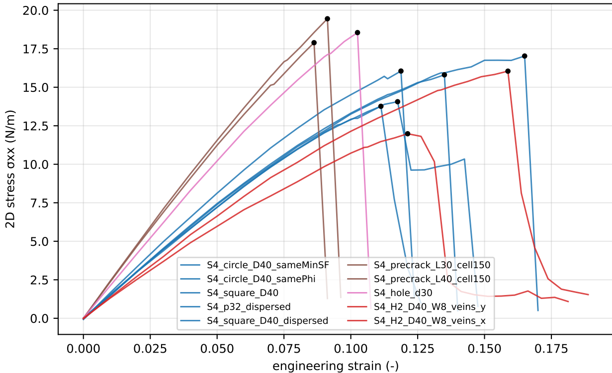
stress-strain curves, stage4_discriminating (10 simulations)
