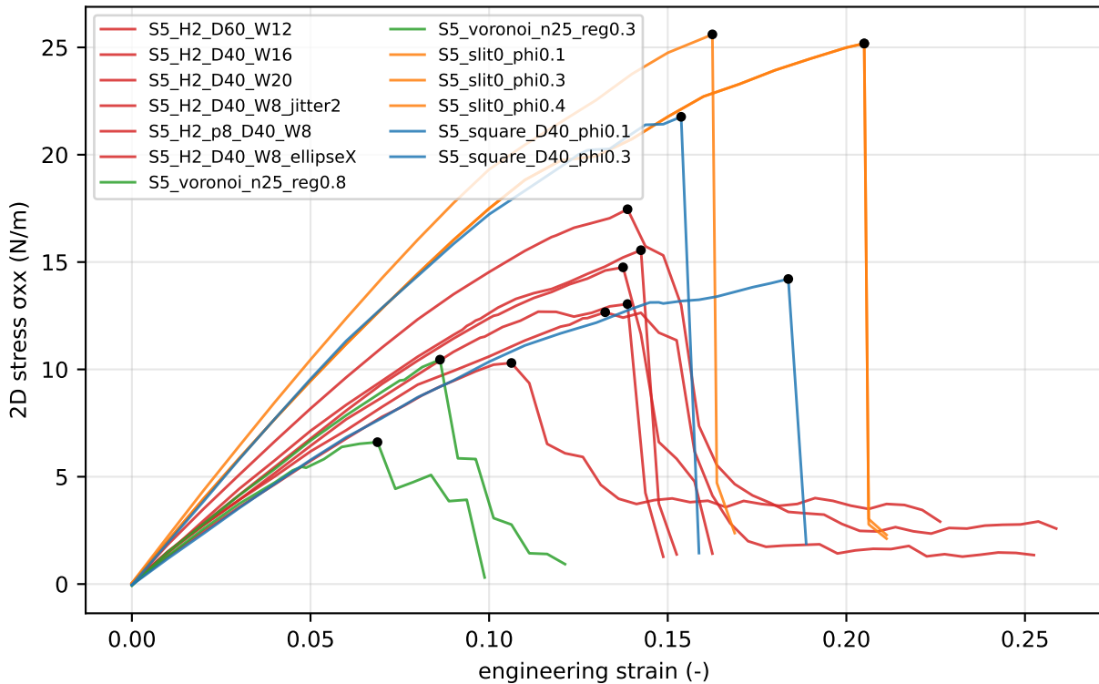
stress-strain curves, stage5_deep (13 simulations)
