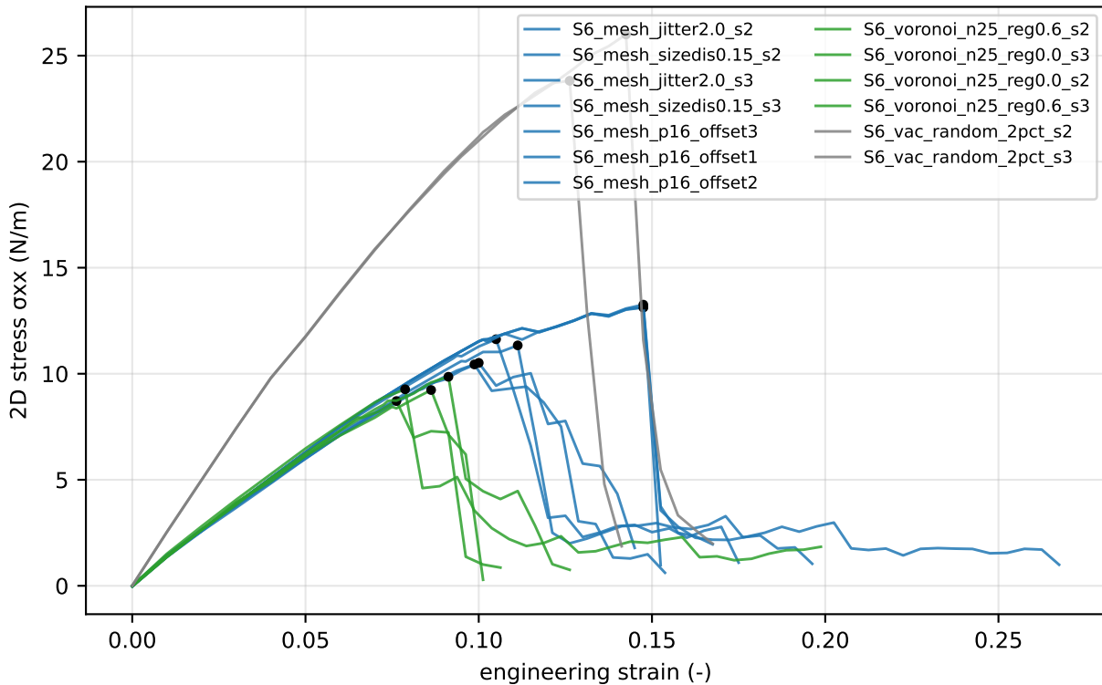
stress-strain curves, stage6_seeds (13 simulations)
