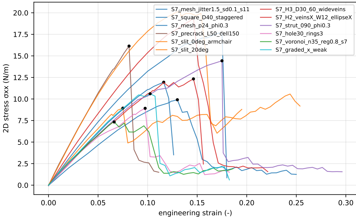
stress-strain curves, stage7_holdouts (12 simulations)
