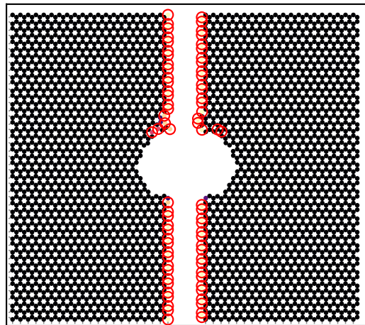
final: \epsilon=0.098 , \sigma=0.8 N/m
