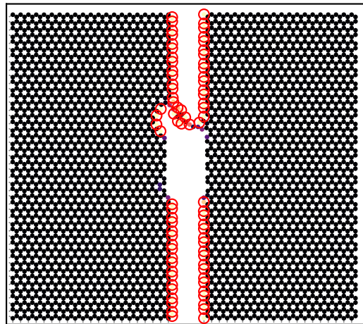
final: \epsilon=0.091 , \sigma=1.1 N/m
