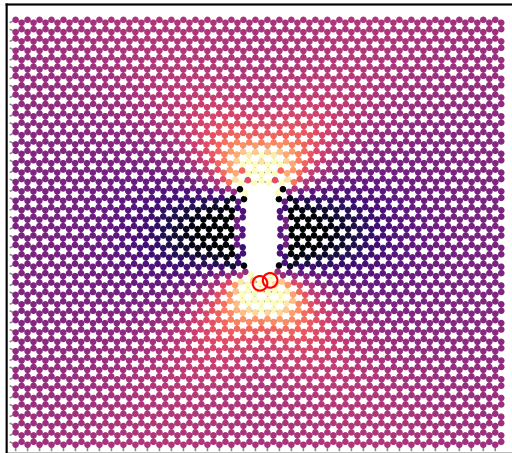
peak load: \epsilon=0.086 , \sigma=18.5 N/m
