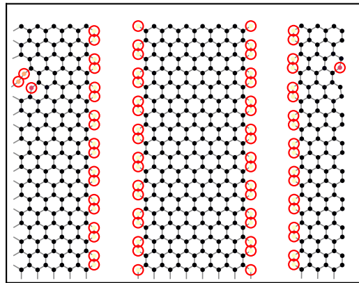
final: \epsilon=0.271 , \sigma=0.2 N/m
