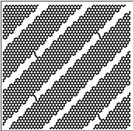
relaxed: \epsilon=0.000 , \sigma=-0.0 N/m
