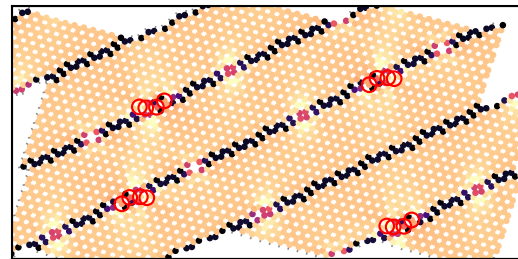
final: \epsilon=0.324 , \sigma=18.5 N/m
