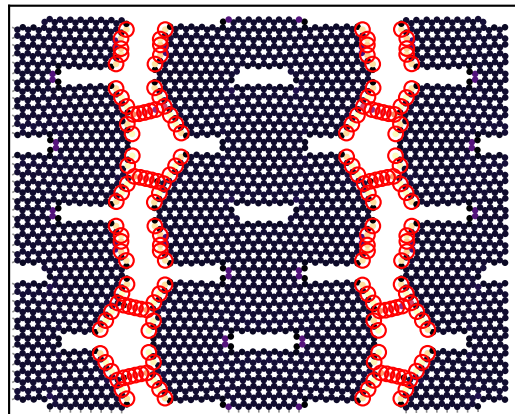
final: \epsilon=0.169 , \sigma=2.4 N/m
