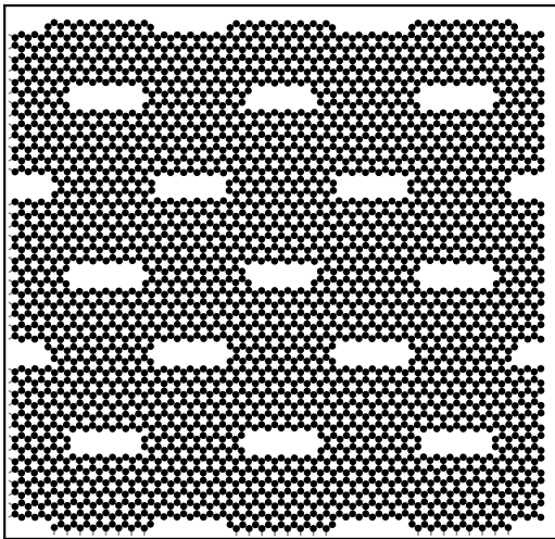
relaxed: \epsilon=0.000 , \sigma=0.0 N/m
