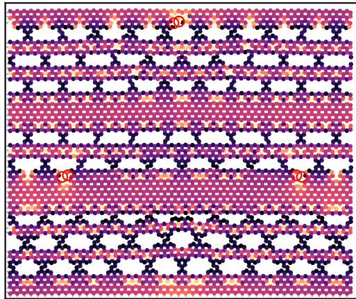
peak load: \epsilon=0.146 , \sigma=19.4 N/m
