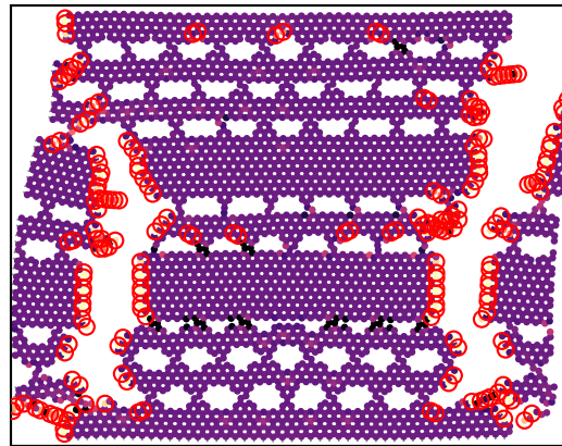
final: \epsilon=0.221 , \sigma=1.6 N/m
