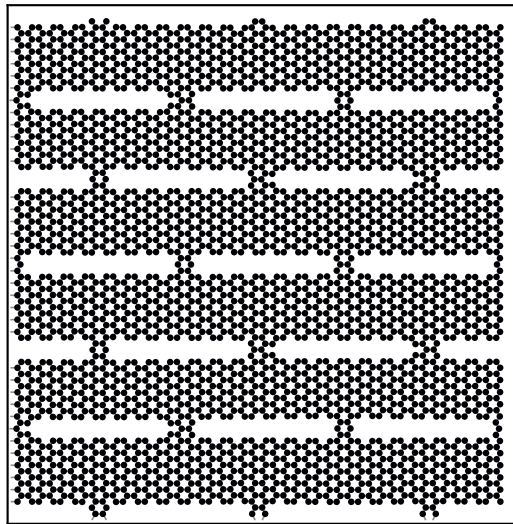
peak load: \epsilon=0.000 , \sigma=-0.1 N/m
