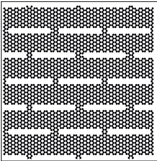
relaxed: \epsilon=0.000 , \sigma=-0.1 N/m
