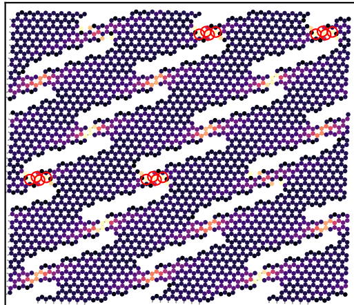
peak load: \epsilon=0.075 , \sigma=8.9 N/m
