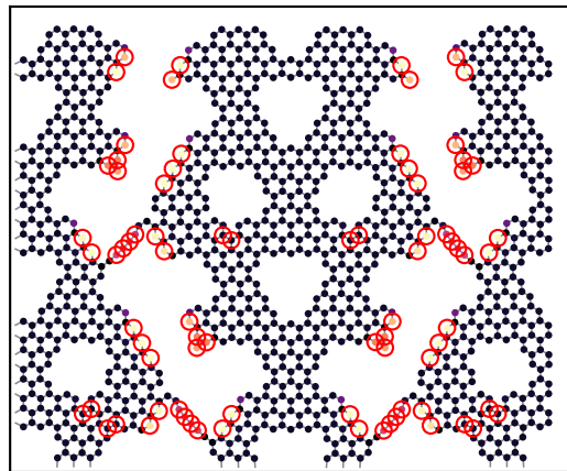
final: \epsilon=0.219 , \sigma=0.5 N/m
