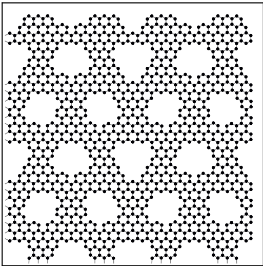
relaxed: \epsilon=0.000 , \sigma=0.1 N/m
