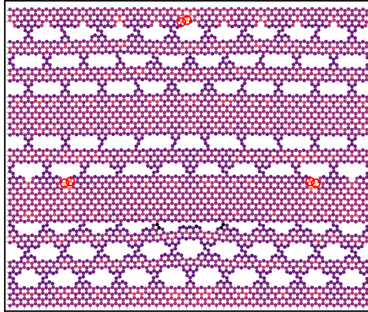
peak load: \epsilon=0.146 , \sigma=19.4 N/m
