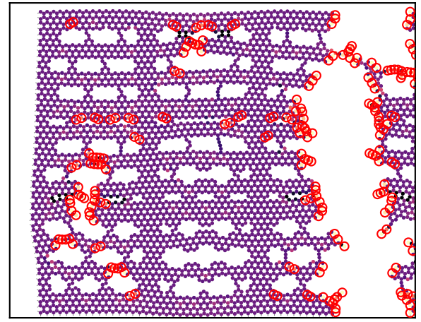
final: \epsilon=0.259 , \sigma=2.6 N/m
