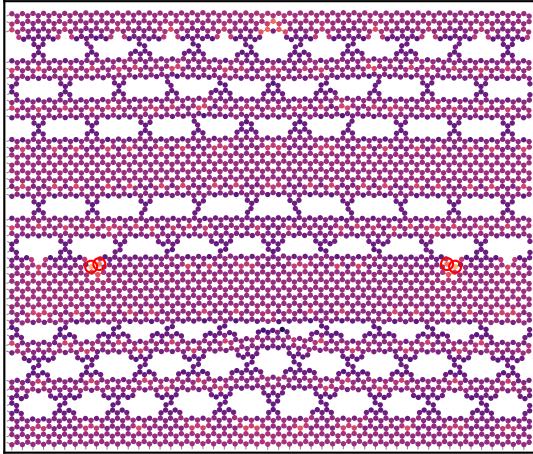
first damage: \epsilon=0.141 , \sigma=19.0 N/m
