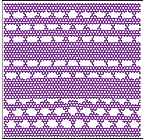
H2: load-elongated fine pores + load-parallel veins (holdout, 19.4 N/m) relaxed: \epsilon=0.000 , \sigma=-0.1 N/m
