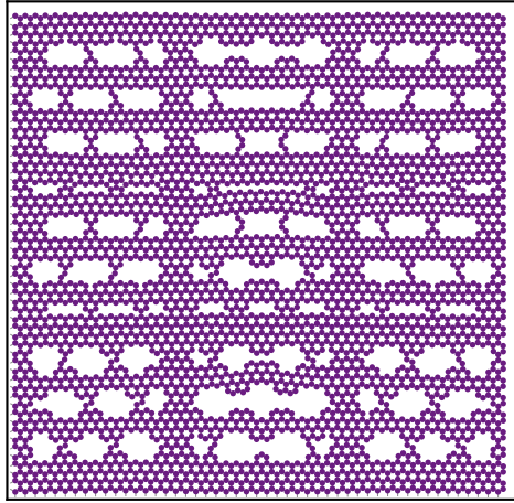
H2: load-elongated fine pores + load-parallel veins (holdout, 19.4 N/m) relaxed: \epsilon=0.000 , \sigma=-0.1 N/m
