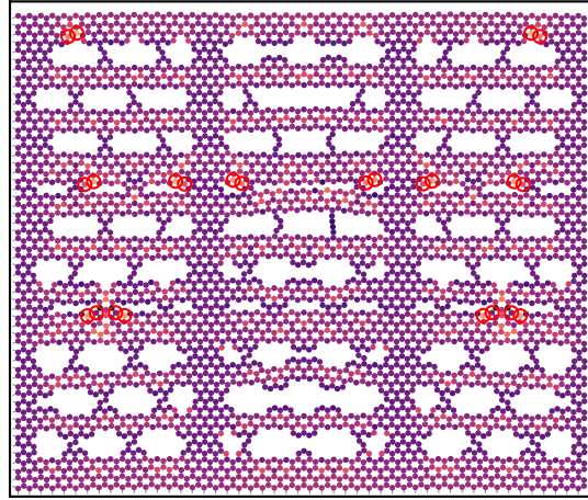
peak load: \epsilon=0.139 , \sigma=17.5 N/m
