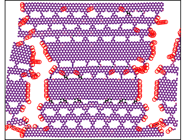
final: \epsilon=0.221 , \sigma=1.6 N/m
