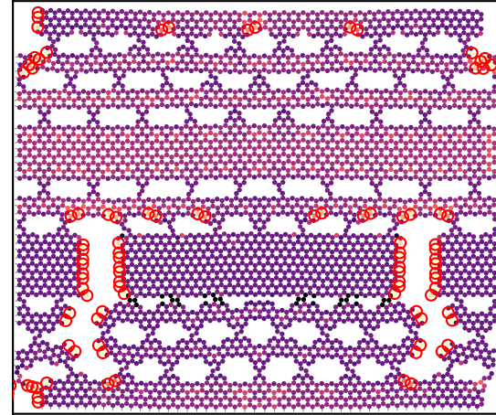
post peak: \epsilon=0.156 , \sigma=11.8 N/m
