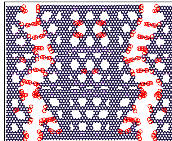
final: \epsilon=0.206 , \sigma=2.3 N/m
