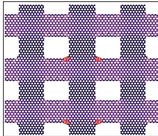
first damage: \epsilon=0.135 , \sigma=15.9 N/m
