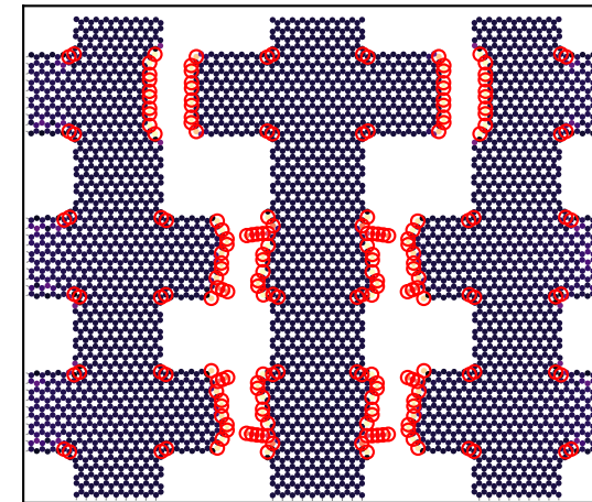
post peak: \epsilon=0.170 , \sigma=2.7 N/m
