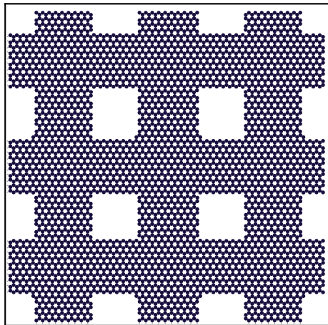
two-level nested mesh (D=40 A, W=8 A) relaxed: \epsilon=0.000 , \sigma=0.0 N/m
