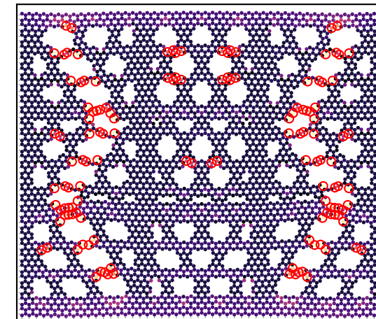
post peak: \epsilon=0.141 , \sigma=8.8 N/m
