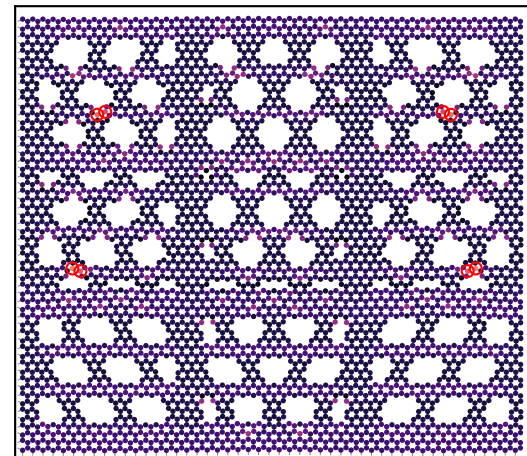
first damage: \epsilon=0.111 , \sigma=12.1 N/m
