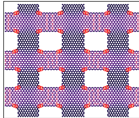
peak load: \epsilon=0.165 , \sigma=17.0 N/m
