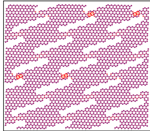
first damage: \epsilon=0.065 , \sigma=8.1 N/m
