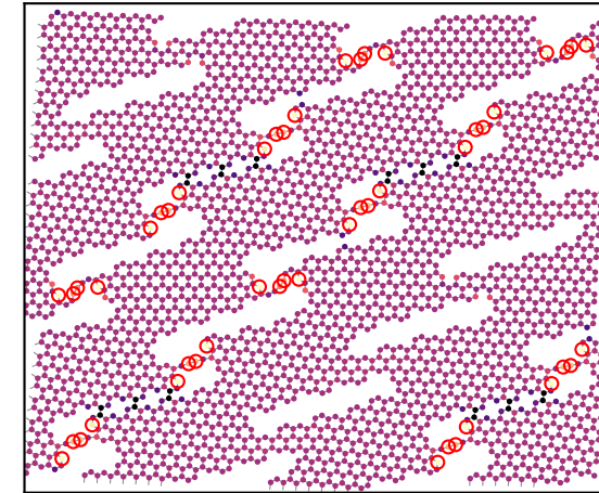
post peak: \epsilon=0.085 , \sigma=5.1 N/m
