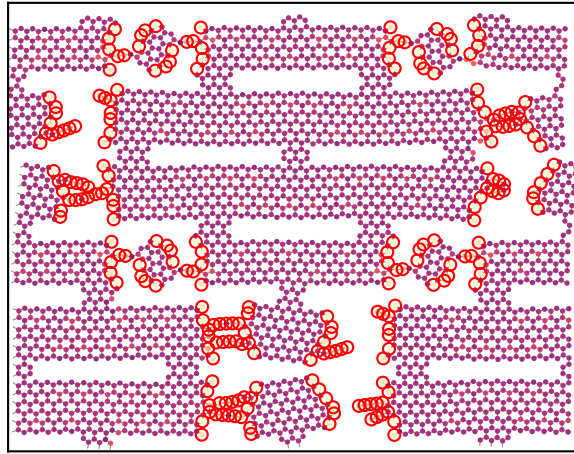
first damage: \epsilon=0.204 , \sigma=5.0 N/m
