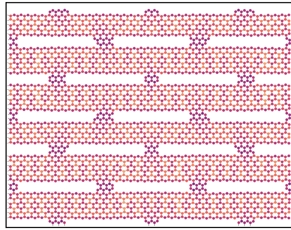
peak load: \epsilon=0.203 , \sigma=25.4 N/m
