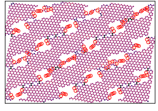
final: \epsilon=0.195 , \sigma=8.8 N/m
