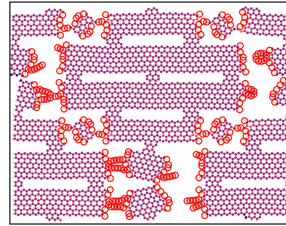
post peak: \epsilon=0.209 , \sigma=3.2 N/m
