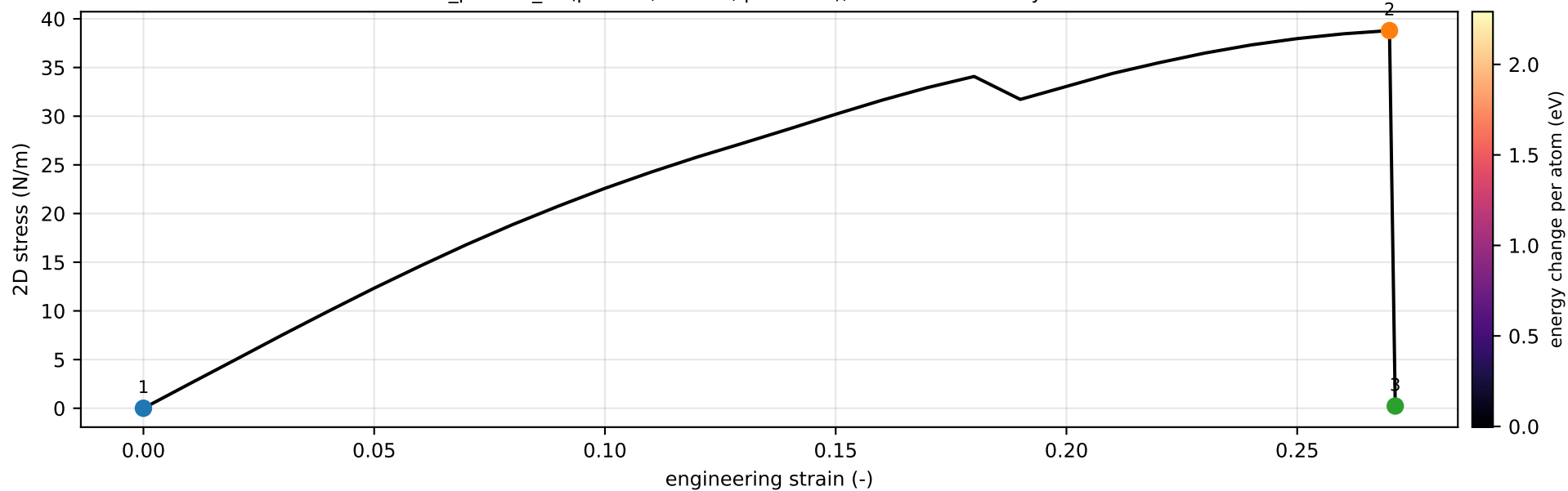
S1_pristine_zz (pristine, N=576, \phi=0.00 ); frames selected by events
