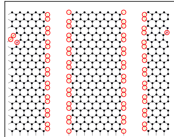
3. first damage = major propagation = post peak = final \varepsilon=0.2713 , \sigma=0.2 N/m, broken=38
