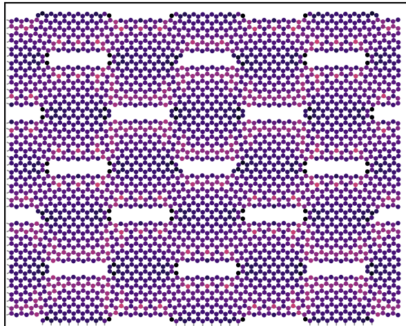
2. pre damage = peak load \varepsilon=0.1625 , \sigma=25.6 N/m, broken=0
