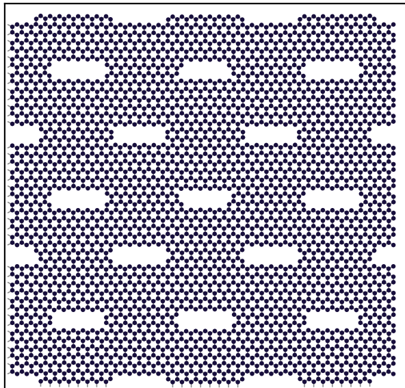
1. relaxed \varepsilon=0.0000 , \sigma=0.0 N/m, broken=0
