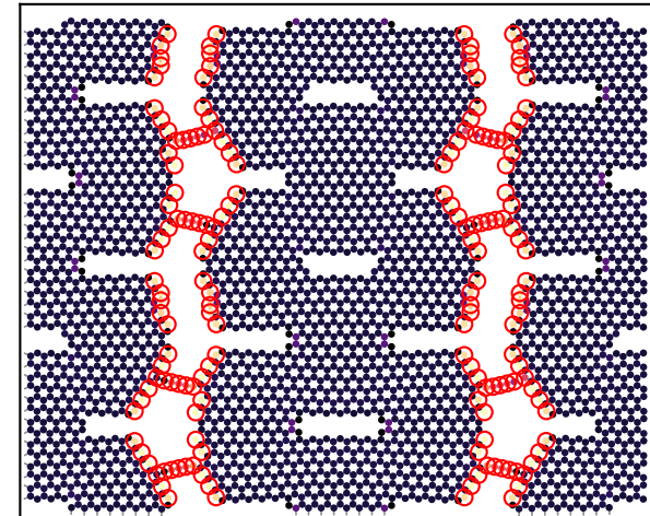
4. post peak = final \varepsilon=0.1688 , \sigma=2.4 N/m, broken=92
