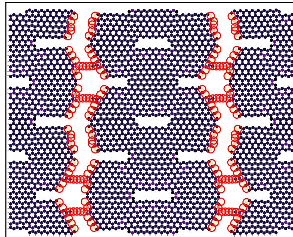
3. first damage = major propagation \varepsilon=0.1638 , \sigma=4.7 N/m, broken=84
