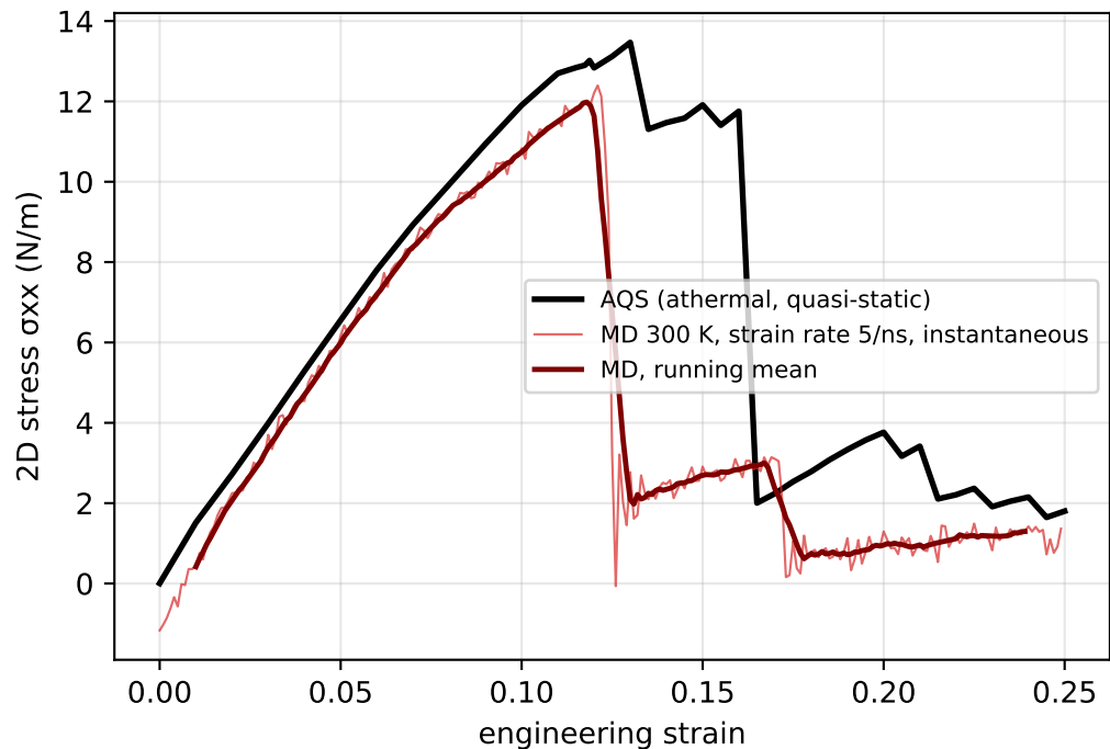
reference nanomesh (N=704): MD vs AQS
