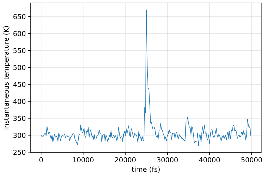
Langevin thermostat, 0.5 fs steps
