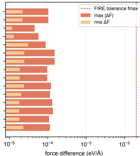
Fast discovery mode (mps float32) vs reference mode (cpu float64) on relaxed, pre-damage, peak-load and post-peak configurations
