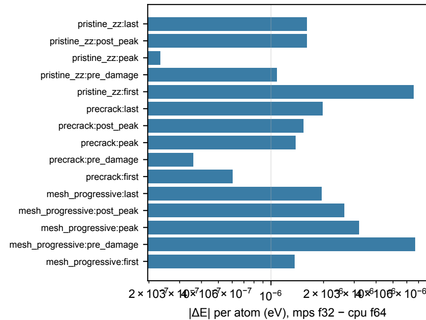
Fast discovery mode (mps float32) vs reference mode (cpu float64) on relaxed, pre-damage, peak-load and post-peak configurations
