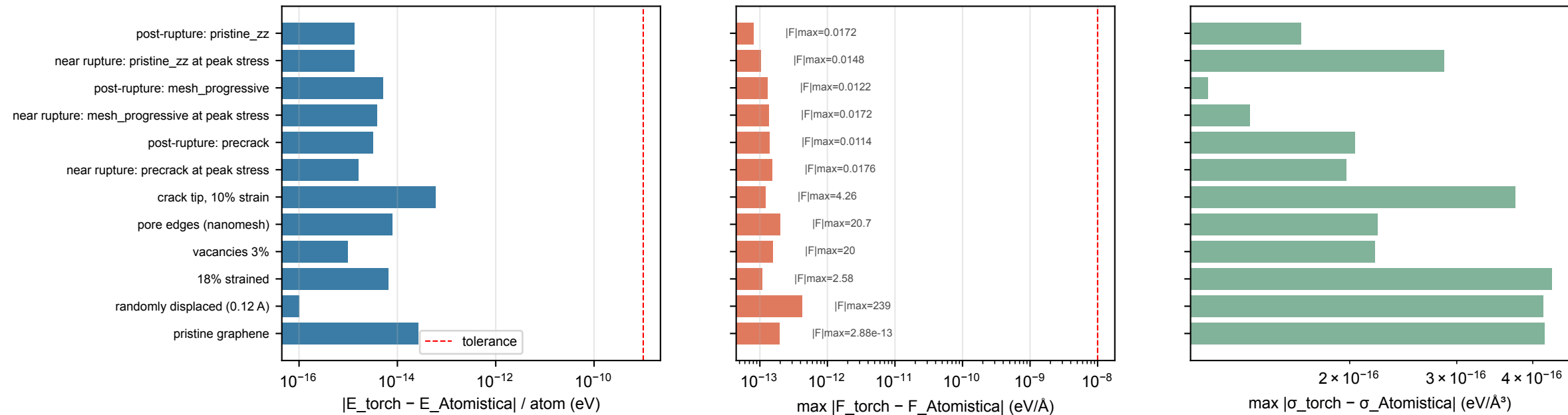
TorchRebo2Scr (cpu float64) vs Atomistica Rebo2Scr: energies, forces and stress for ordinary and difficult configurations
