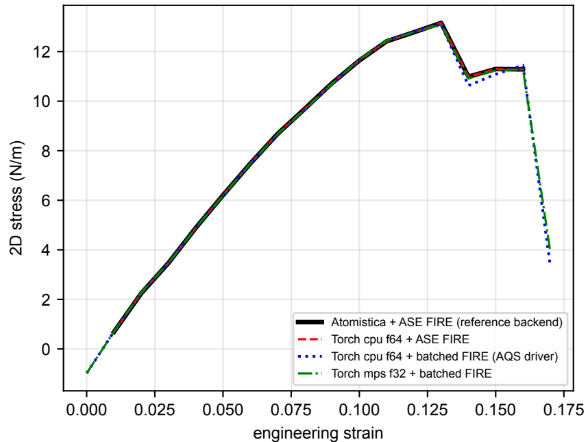
nanomesh (N=704); max |\Delta\sigma| cpu64: 3.60e-01, mps32: 7.76e-02 N/m
