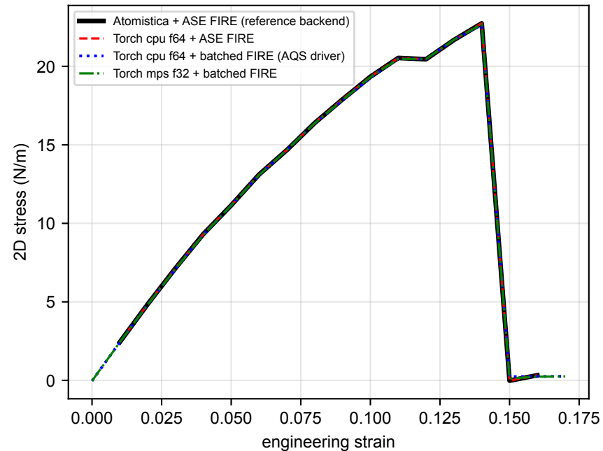
precrack (N=561); max |\Delta\sigma| cpu64: 2.55e-01, mps32: 1.39e-01 N/m
