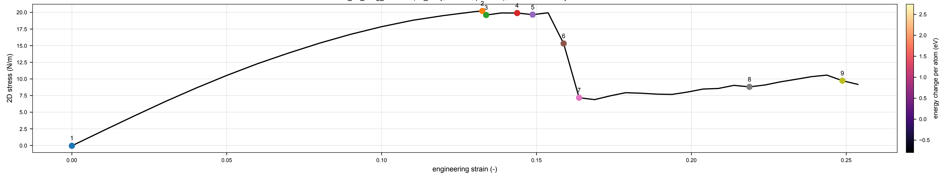
S7_slit_0deg_armchair (slit_array, N=3068, phi=0.19); frames selected by events
