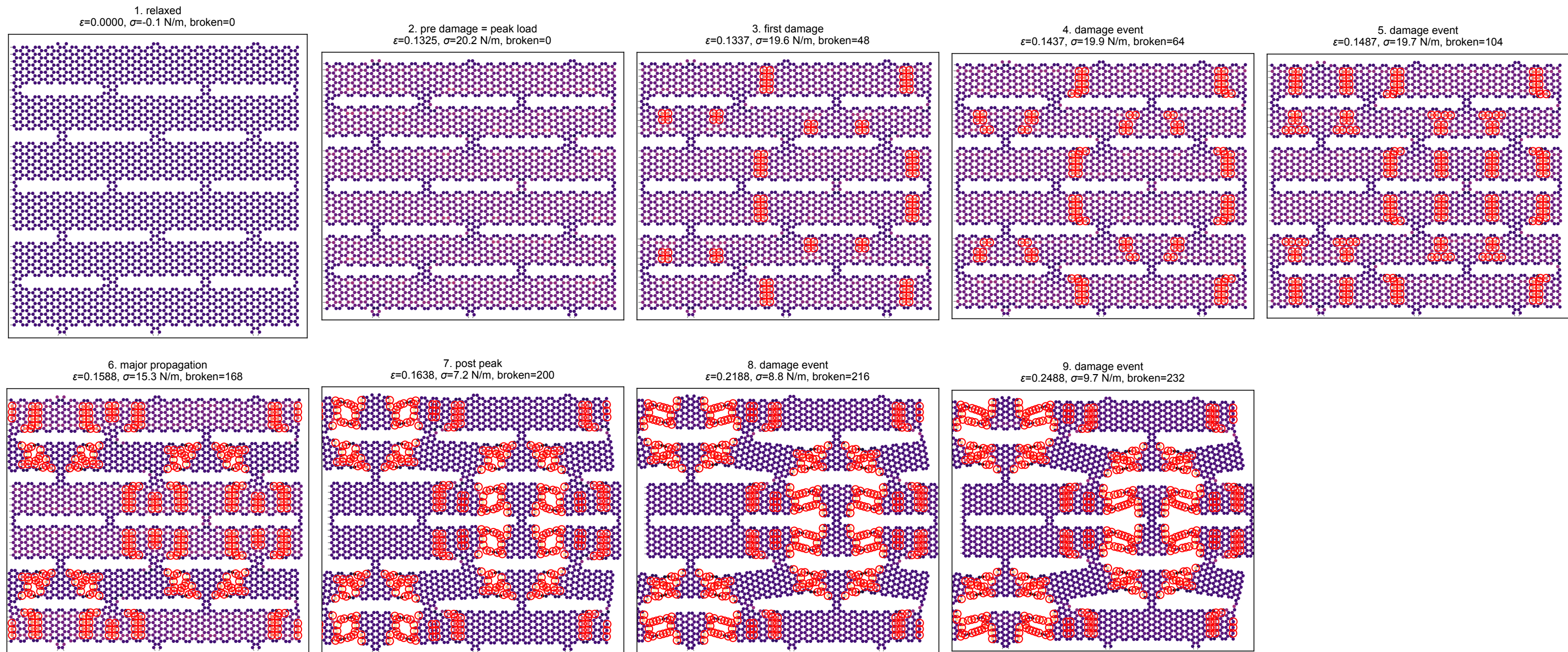
S7_slit_0deg_armchair (slit_array, N=3068, phi=0.19); frames selected by events
