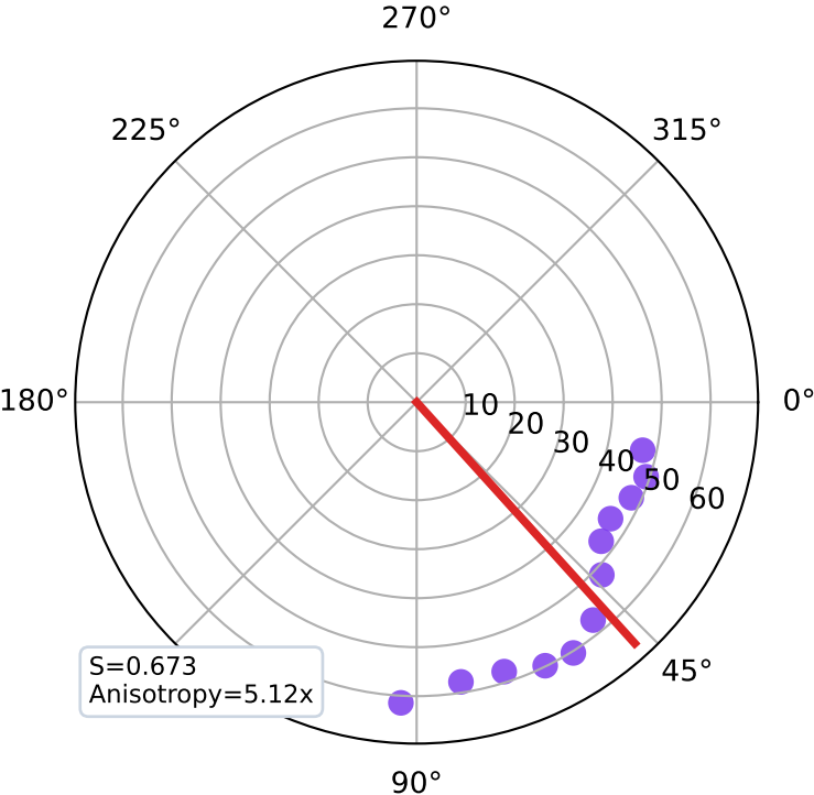
A. Orientation tensor identifies load-bearing axis
