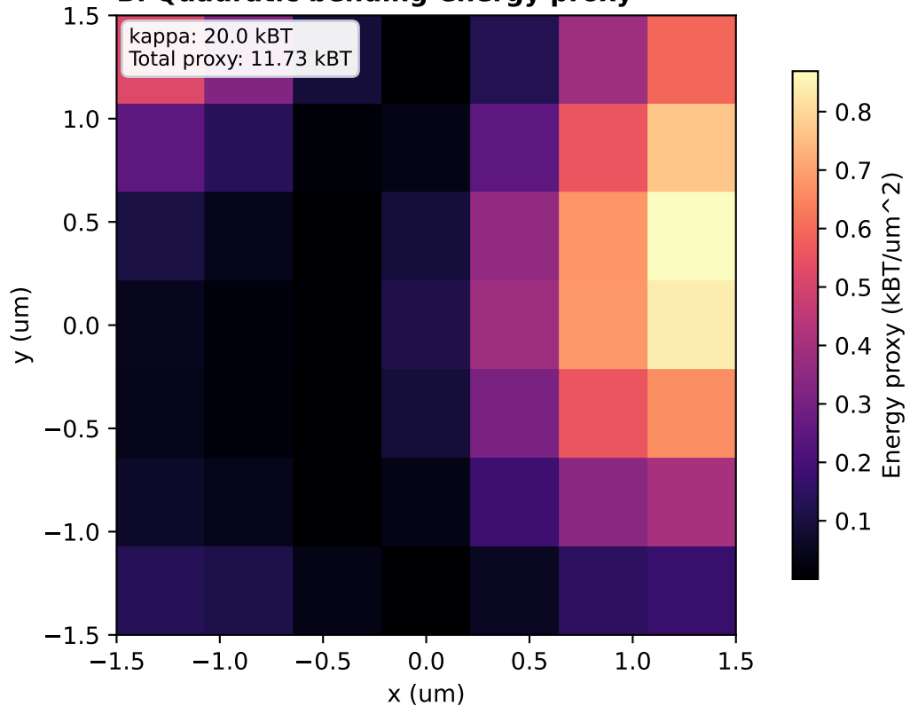
B. Quadratic bending-energy proxy
