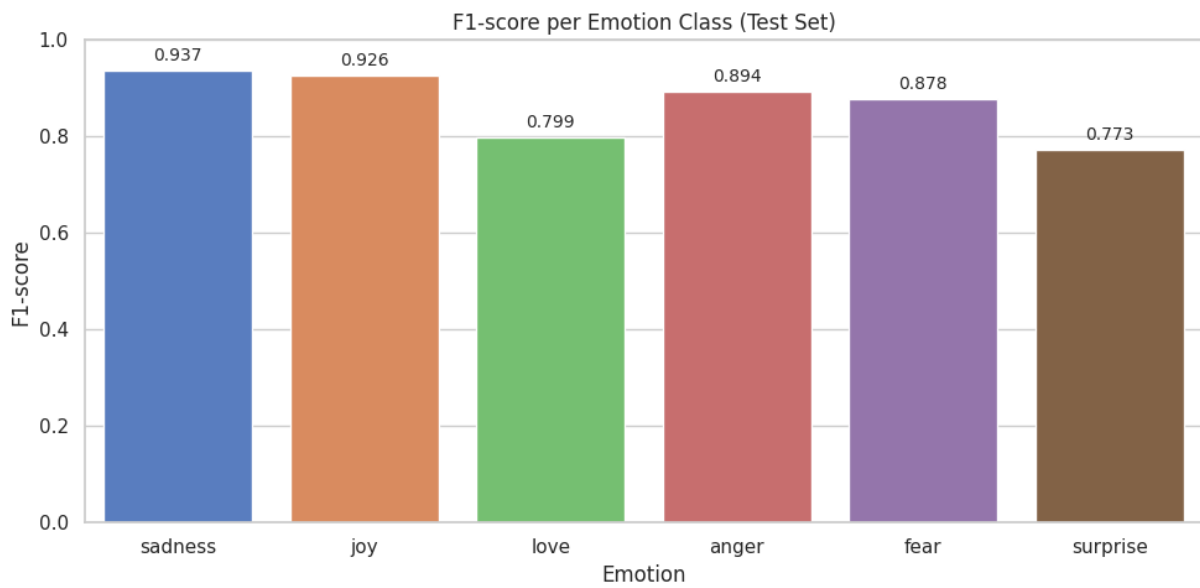
Figure 3: F1-score per emotion class on the test set.
