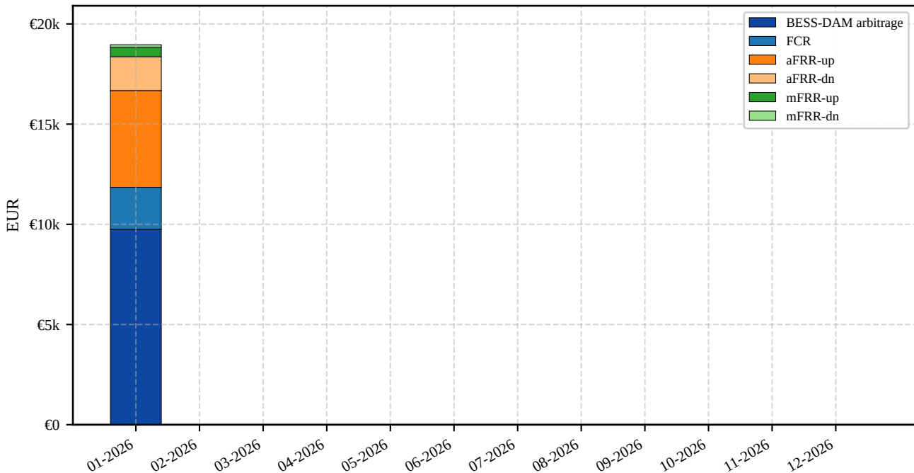
BESS revenue by month (self_consumption; Hybrid PV+BESS) (Year 1)
