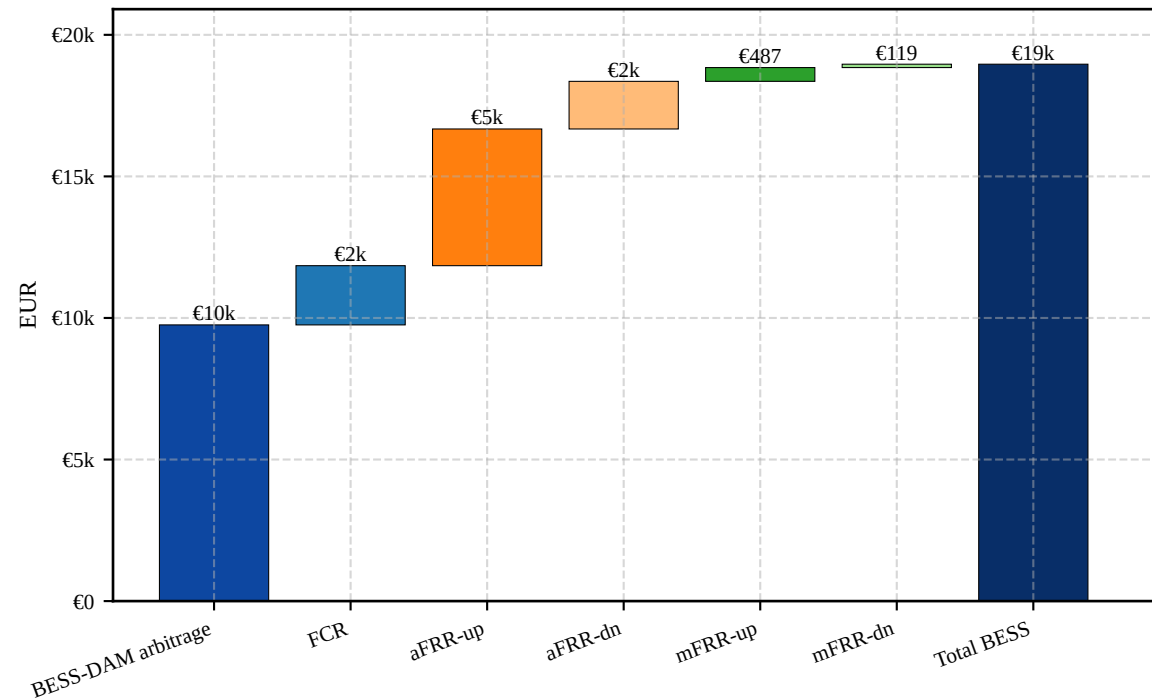
BESS revenue waterfall (self_consumption; Hybrid PV+BESS) (Year 1)
