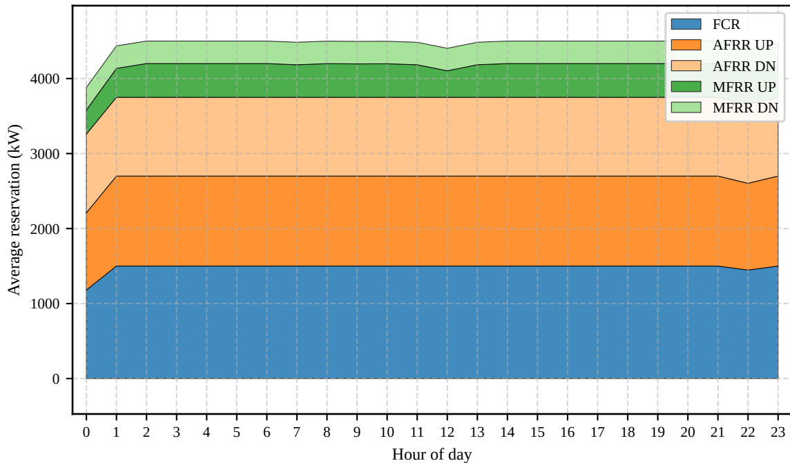
Balancing reservation profile (self_consumption; Hybrid PV+BESS) (Year-1 average)
