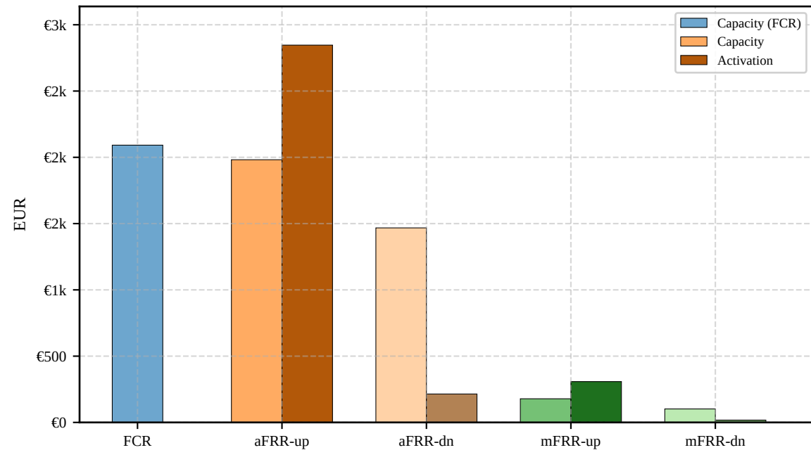
Balancing revenue: capacity vs activation (self_consumption; Hybrid PV+BESS) (Year 1)
