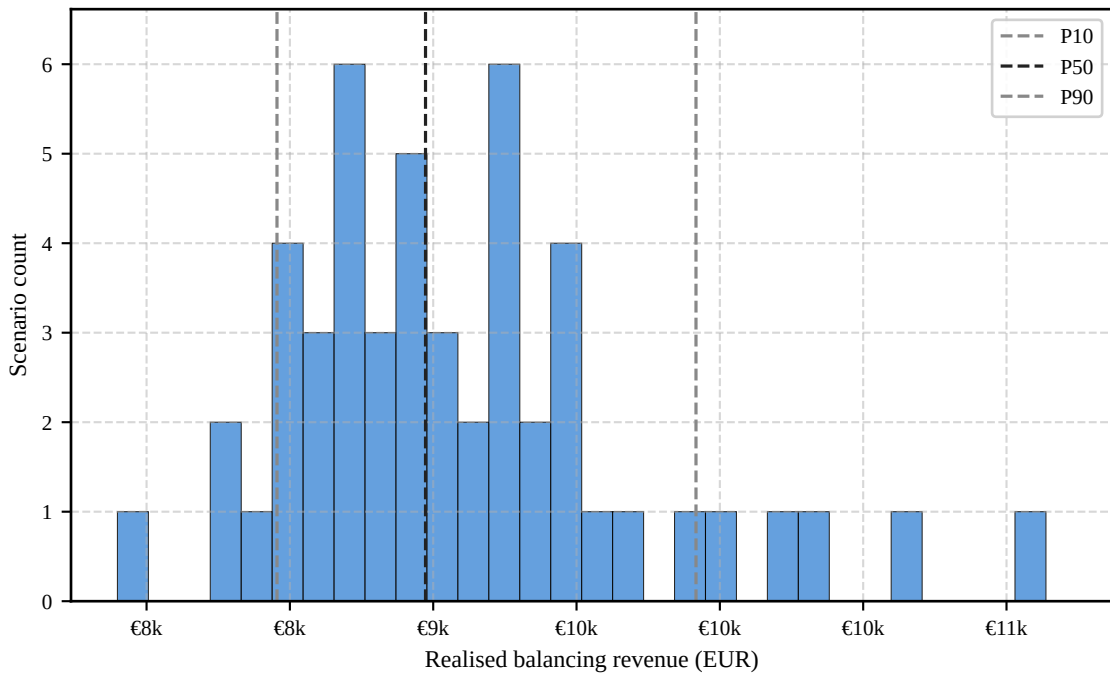
Balancing revenue — Monte Carlo distribution (self_consumption; Hybrid PV+BESS)
