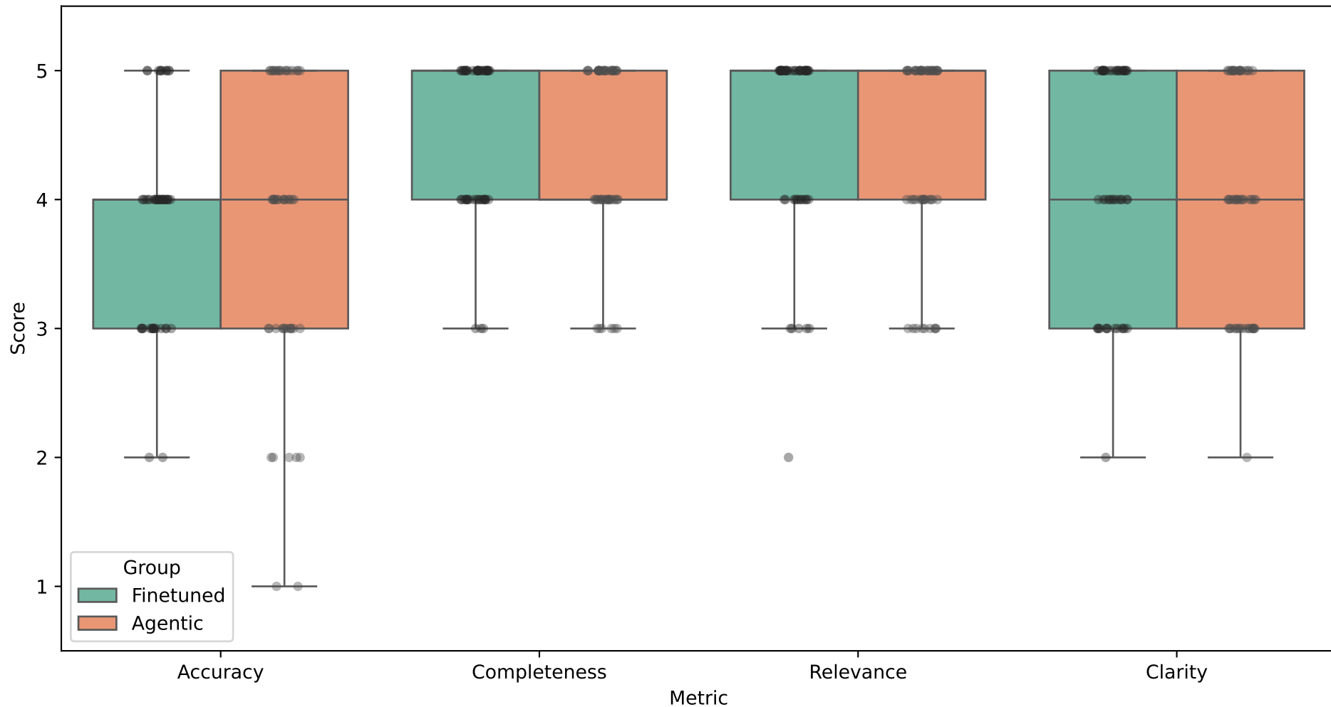
Human Scores: Agentic vs Finetuned (Box = Distribution, Dots = 5 Students)
