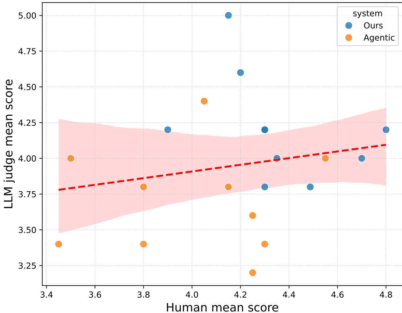
Human--LLM Mean Pointwise Alignment Pearson r = 0.19 , Spearman \rho = 0.15
