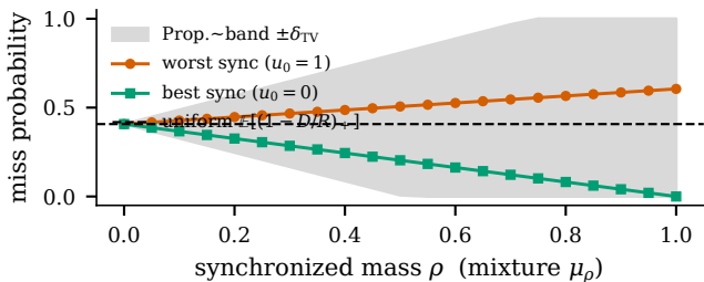
(a) perturbation bound, R = 5
