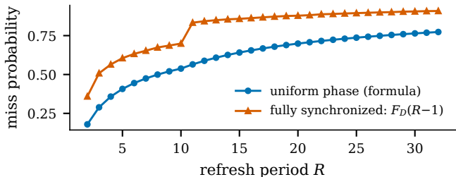
(b) worst-case ceiling across R
