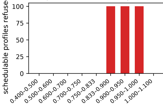
price of the O(1) density test
