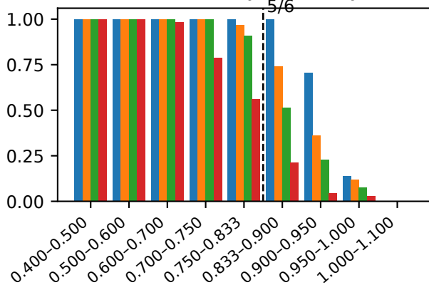
schedulability vs density
