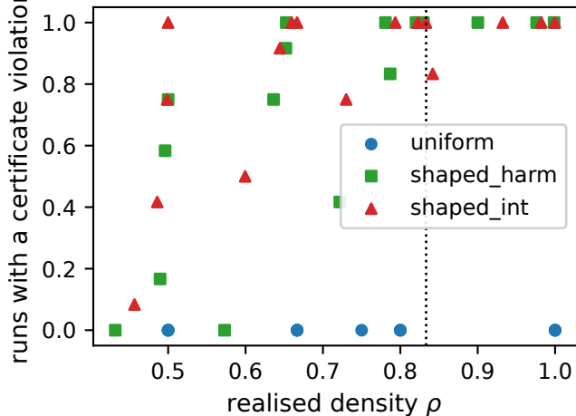
lazy EDF breaks the certificate
