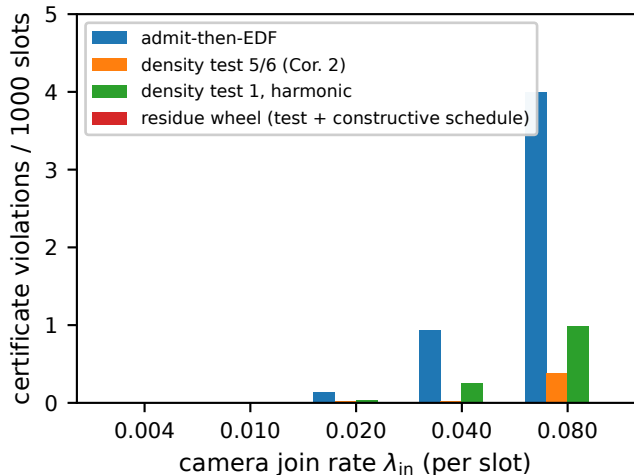
certificate violations under churn
