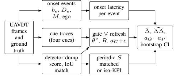
Fig. 1. Offline replay pipeline. Both policies are replayed on the same detector dump and the same cue traces; the gate pays the cue cost c on every frame and the periodic competitor is given the same total activation (matched cost) or the activation it needs to reach a latency-miss target (iso-KPI). All channel parameters and thresholds come from the TRAIN split; the TEST split is replayed once with the frozen values.
