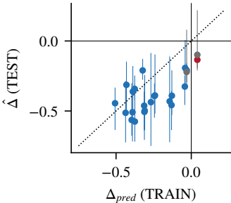
H3/H5: Spearman 0.62
