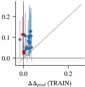
H8: Spearman 0.20
