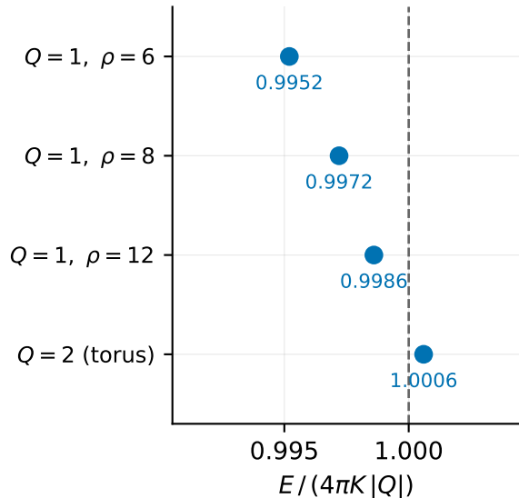
(b) Saturation of the bound
