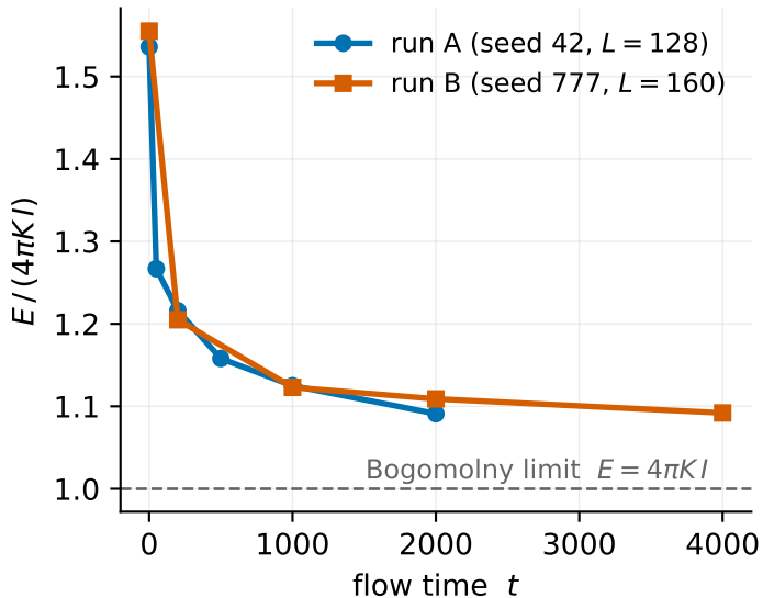
(a) Dynamical quantization under the Nullivance flow
