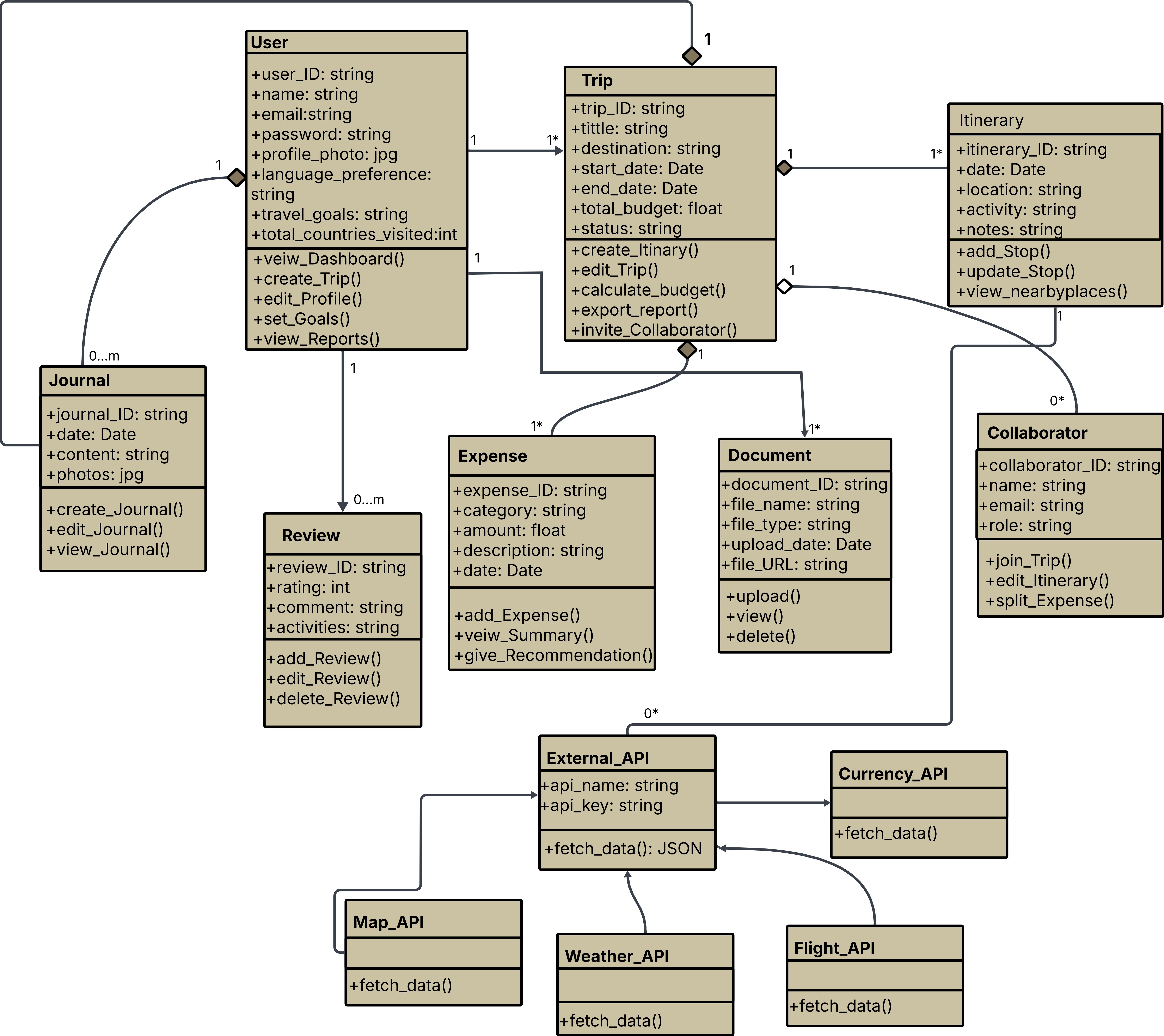
Class Diagram of Group 3 (TripSync: Plan, Pack and Go)
