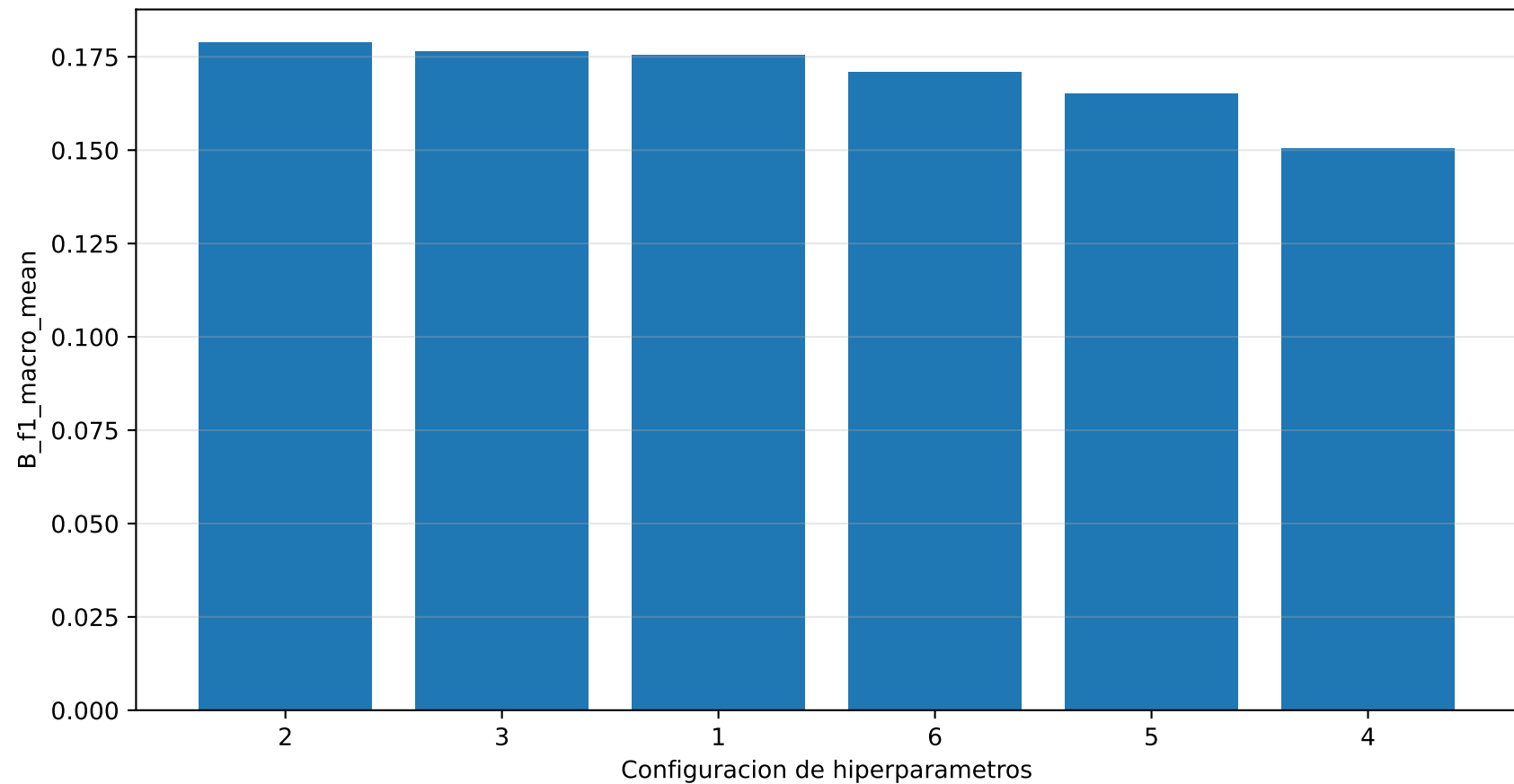
GridSearch CV
