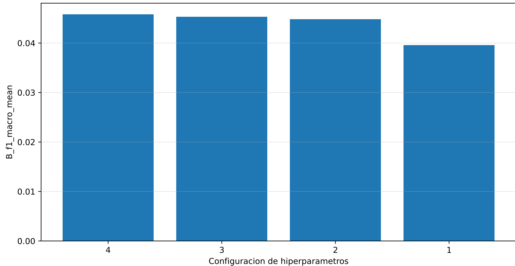
GridSearch CV
