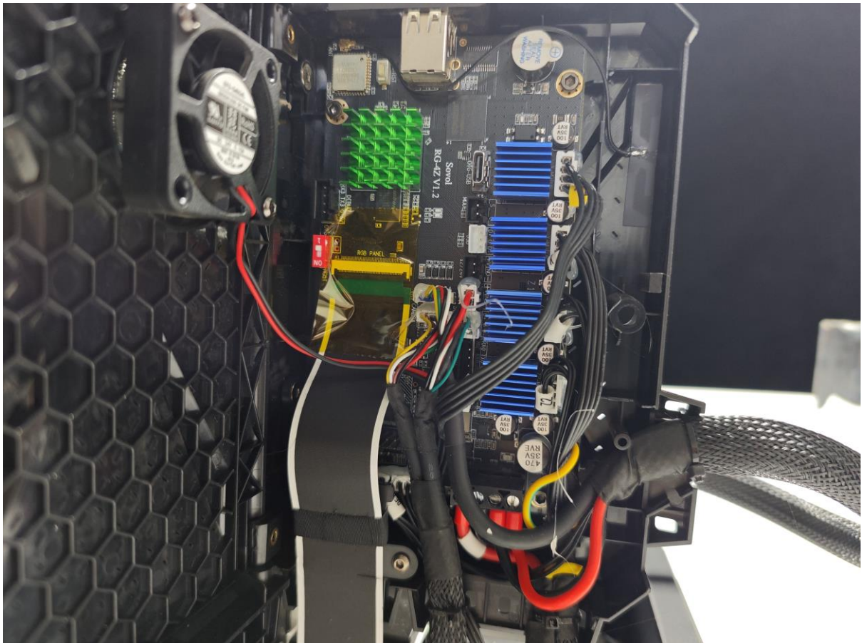
Step 5: Reconnect all the wires to the corresponding ports on the new mainboard.
