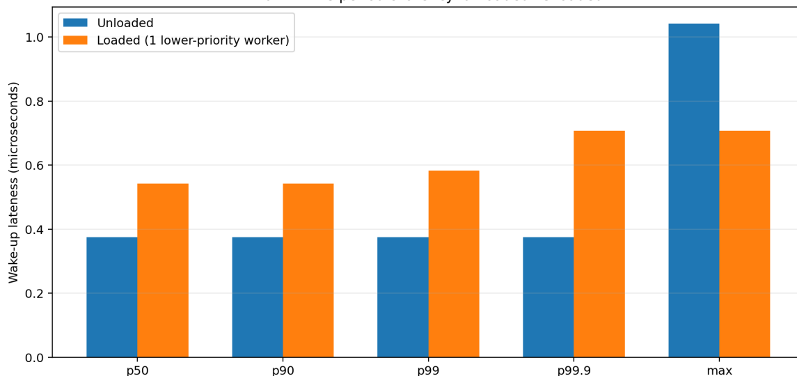
Figure 5. NuttX measured 1 ms wake-up lateness, unloaded and with one lower-priority continuous compute worker.
