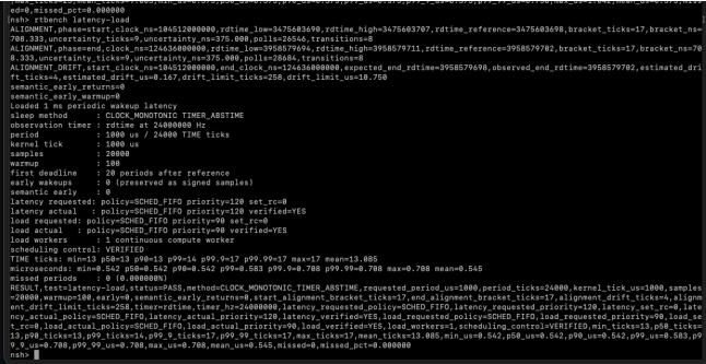
Figure 7. Loaded latency PASS output.
