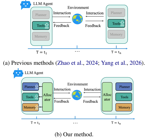
Figure 1: Prior methods fix the harness to one retrieval/update pattern. AEL instead evolves the harness: it learns how to retrieve experience with a fast memory-policy bandit and slow failure-diagnosis reflection.
