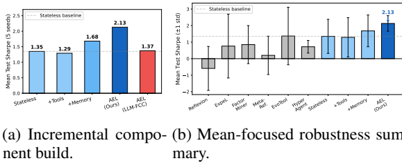
Figure 3: (a) Incremental build (5 seeds): Stateless (1.35) \rightarrow +Memory (1.68) \rightarrow AEL (2.13); adding LLM-FCC credit degrades to 1.37. (b) Robustness: Mean test Sharpe \pm 1 std. AEL has the highest mean (2.13) with the lowest variance among LLM methods.
